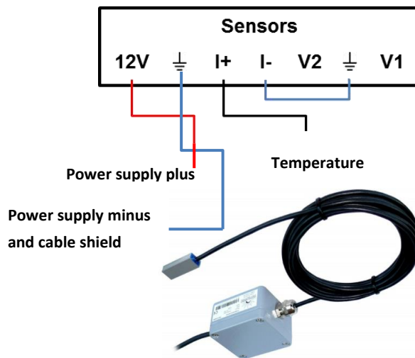
Figure 6: Connecting the Module Temperature Sensor
