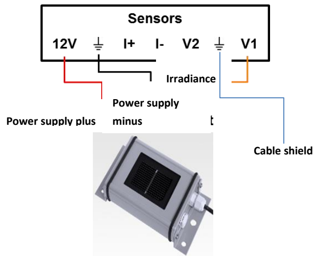
Figure 8: Connecting the Solar Irradiance Sensor
