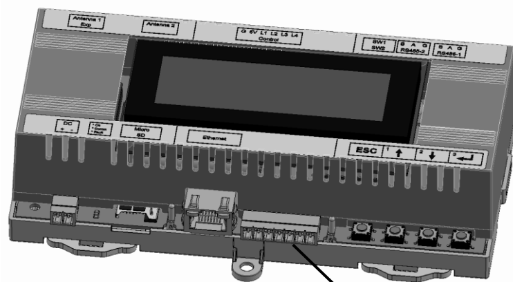
Figure 2: Sensor 7-Pin Terminal Block
