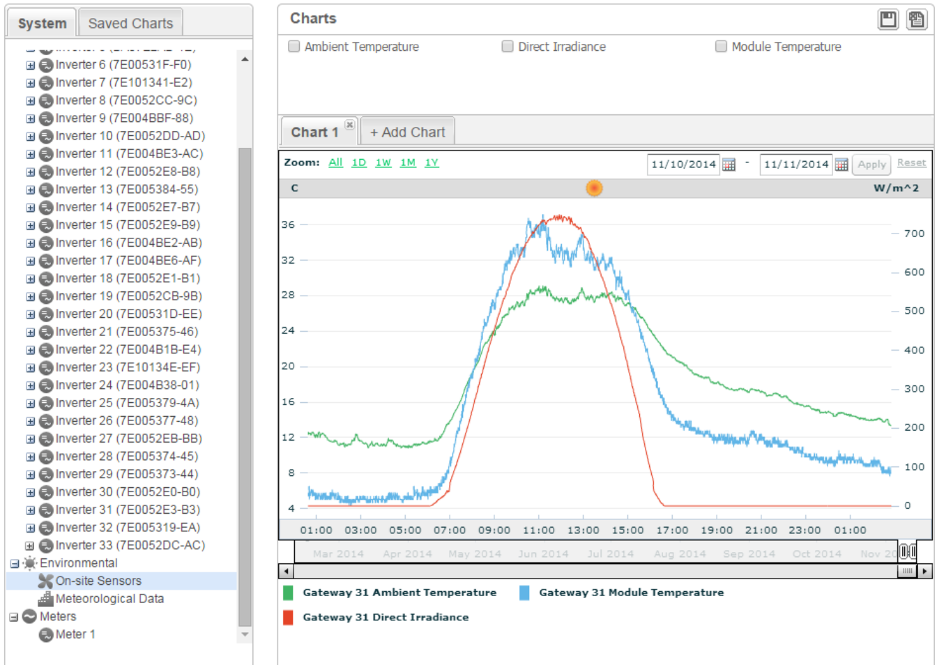
Figure 10: Viewing sensor readings on the monitoring platform
