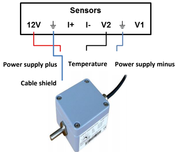
Figure 4: Connecting the Ambient Temperature Sensor
