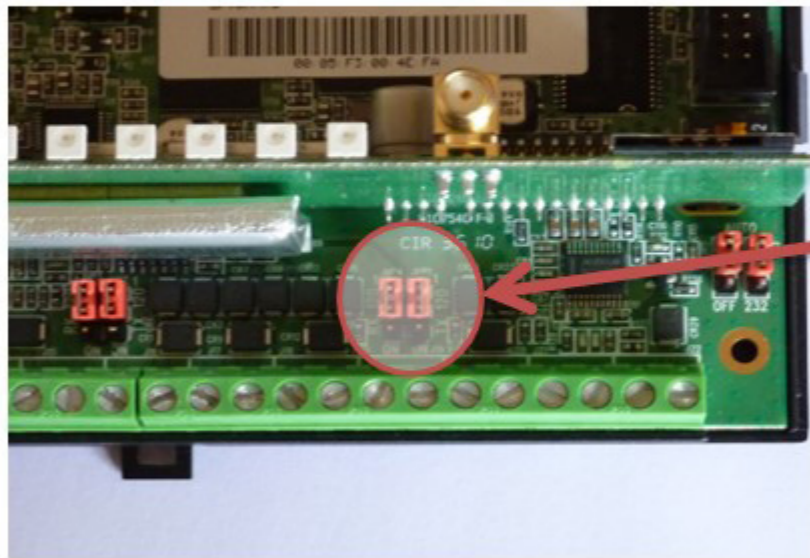
Configuration of bus termination jumper JMP4 and JMP1
